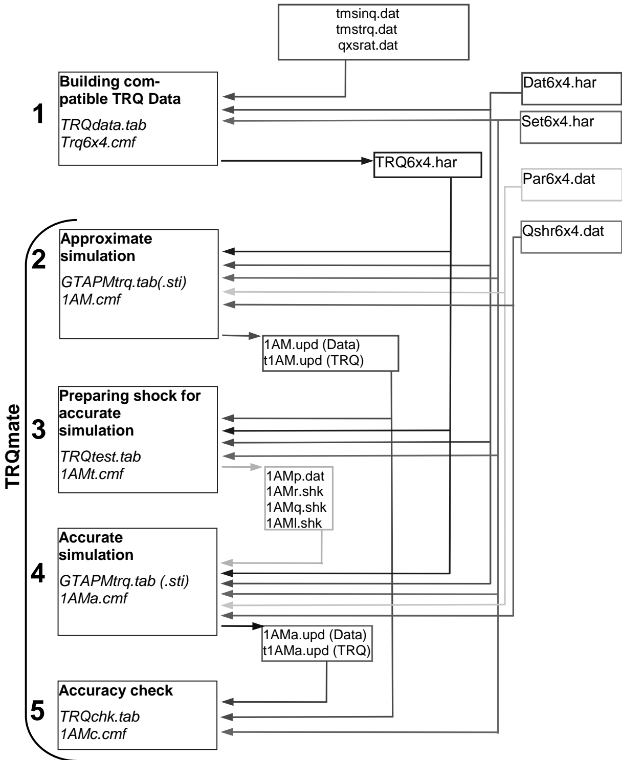
Figure 5: Summary of GEMPACK Procedure for TRQ Simulations
