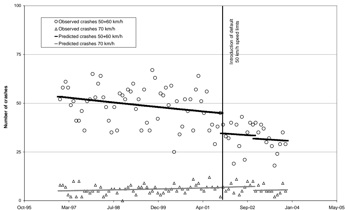
Figure 3-6 Observed and modelled monthly crash frequency in 50 and 60 km/h zones versus 70 km/h speed zones ñ crashes involving MOTORCYCLES
