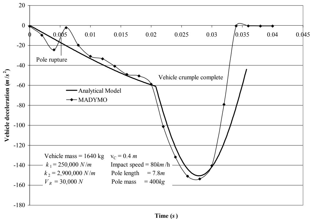
Figure 4 Vehicle deceleration.
