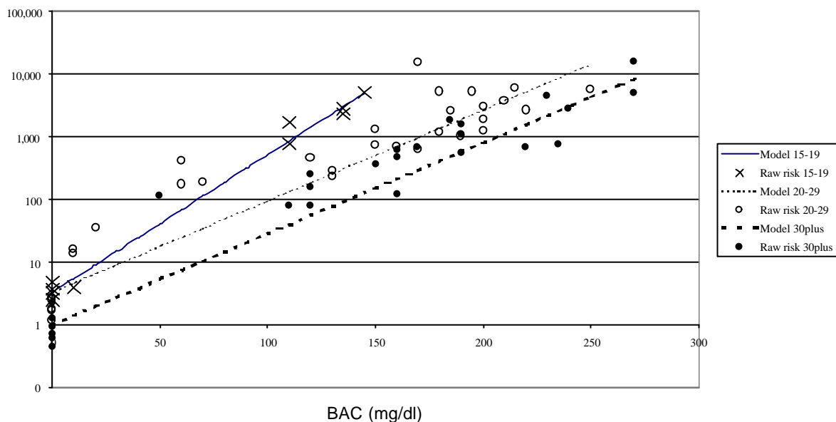
Figure 2: Risk of driver fatal injury by age group relative to drivers aged 30 and over at BAC=0, controlling for location and year
